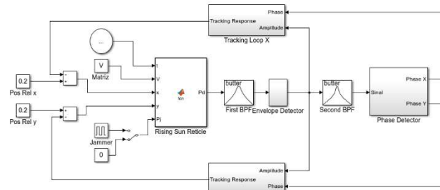
Fig.6 Simulation Model implemented in Simulink.
