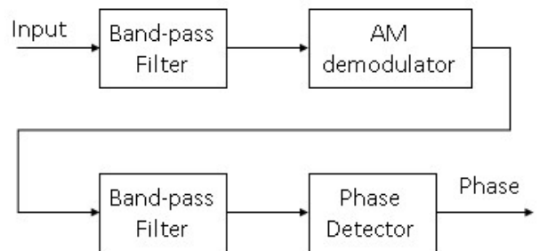
Fig. 4. Signal Processing of Spin-Scan Seeker.
