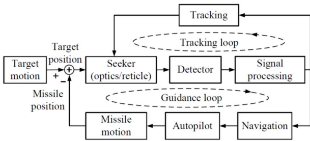
Fig. 1. Typical IR guided missile block diagram [4].
