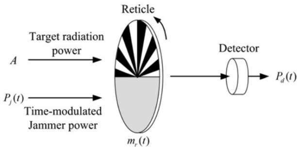
Fig. 2. Rising Sun Reticle Seeker [4].
