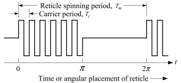
Fig. 3. Detector Output Signal [5].
