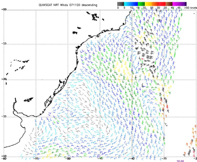
Fig. 7. Wind distribution before the mission.
