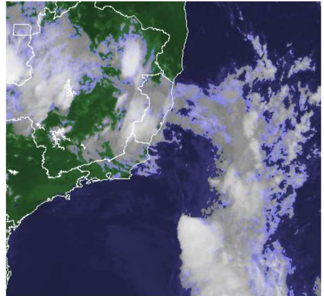
Fig. 8. Cloud formations before the mission.
